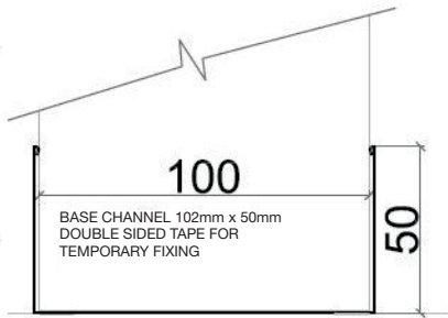
BASE CHANNEL
