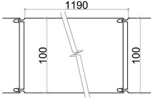
PANEL JOINTS
